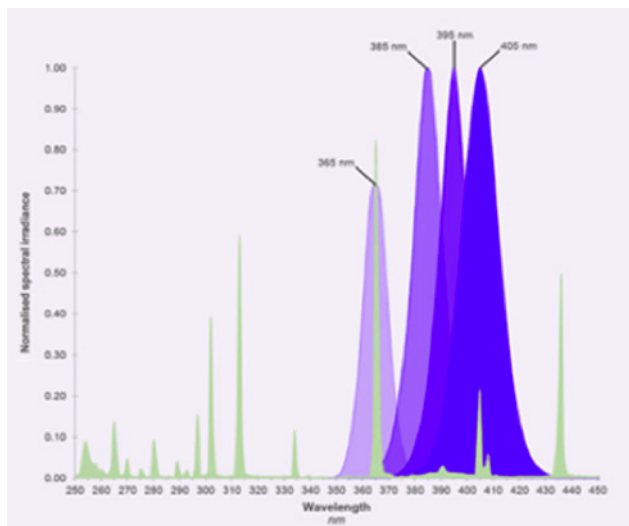
Fig.8 LED-UV is highly efficient around 395 nm wavelength range.
