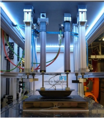
Figure 1. Forming tool “double dome” at IFB
