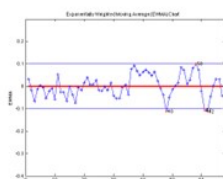
Figure 5c: Inkjet \Delta b^* EWMA chart
