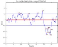
Figure 4a: Offset \Delta L^* EWMA chart
