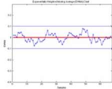
Figure 5a: Inkjet \Delta L^* EWMA chart
