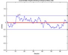
Figure 5b: Inkjet \Delta a^* EWMA chart
