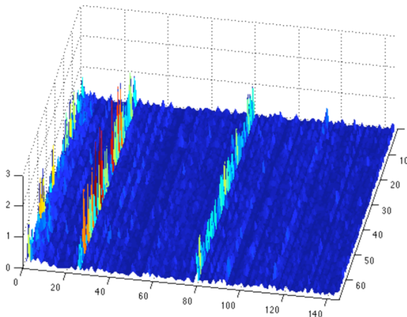
Figure 6a: Inkjet variability (X – Patch#, Y – Sample#, Z – \Delta E )
