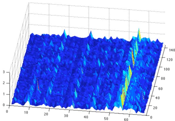
Figure 6b: Offset variability (X – Patch#, Y – Sample#, Z – \Delta E )
